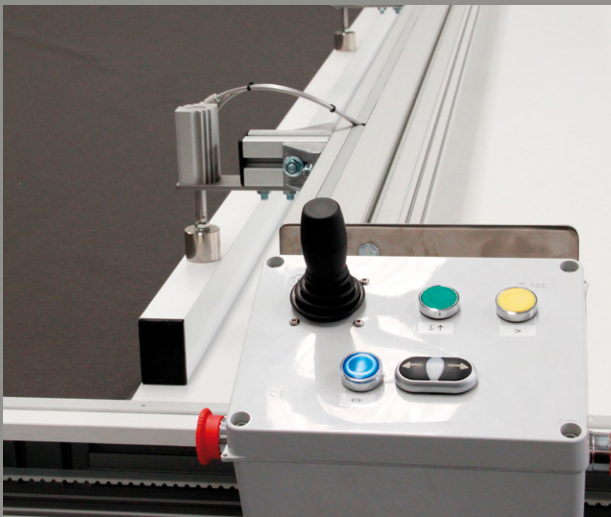
Secondary control and Joystick (Flexicut Plus) / Control secundario y Joystick (Flexicut Plus)
