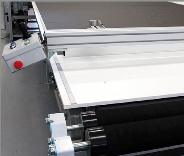
Winding device / Dispositivo de enrollado
